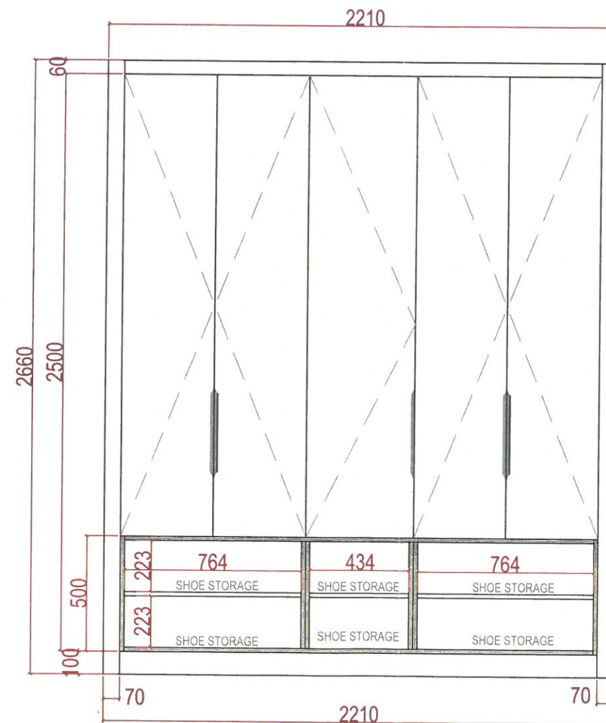
WARDROBE -1 MADAM'S WARDROBE- FRONT VIEW
