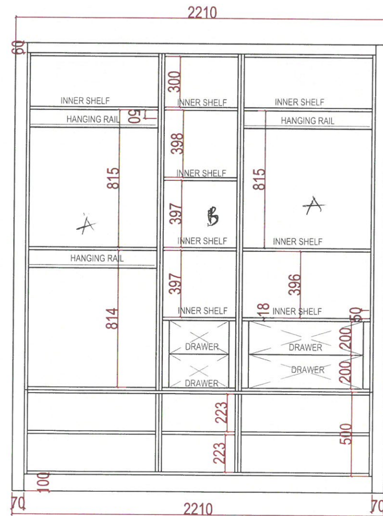
WARDROBE -1 MADAM'S WARDROBE- INNER VIEW
