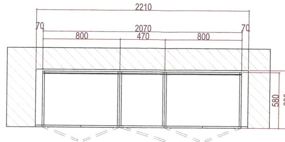
WARDROBE -1 MADAM'S WARDROBE LAYOUT
